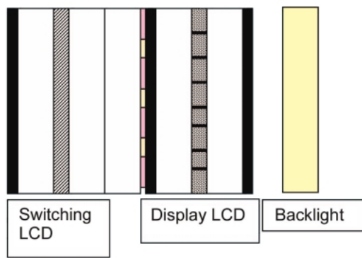
Fig. 5 Display configuration.
