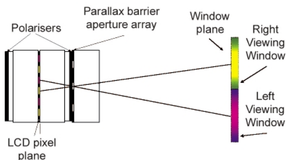
Fig. 3 Parallax barrier display.
